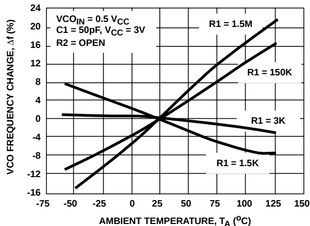
FIGURE 23. HC4046A TYPICAL CHANGE IN VCO FREQUENCY vs AMBIENT TEMPERATURE AS A FUNCTION OF R1 ( V_{CC} = 3V )
