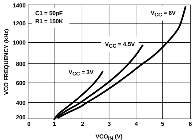
FIGURE 21. HC4046A TYPICAL VCO FREQUENCY vs V_{CO\_IN} ( R1 = 150k\Omega , C1 = 50pF )
