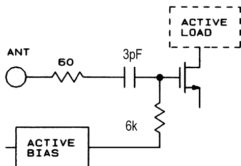
Figure 1 ANT Pin
