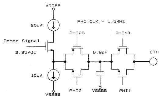
Figure 2 CTH Pin
